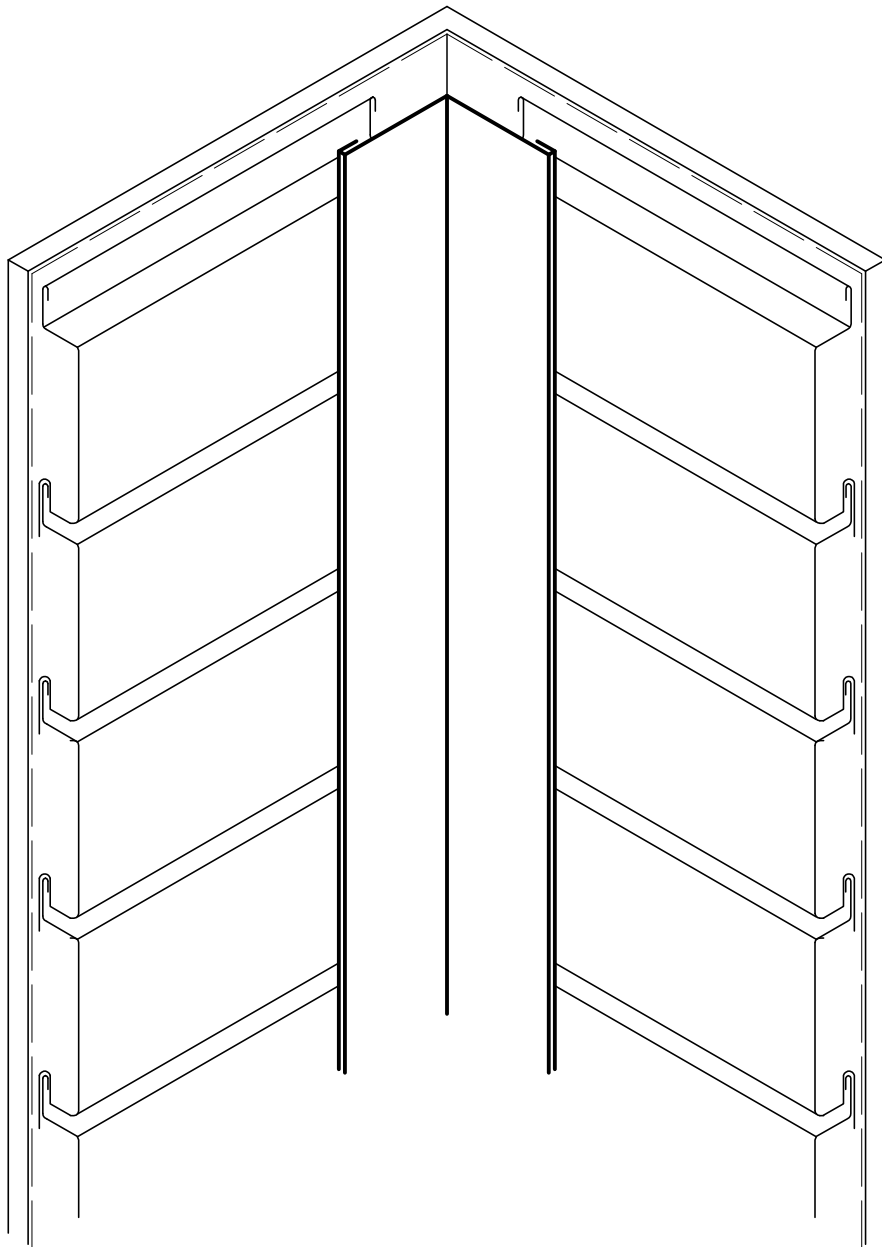
3 INSIDE CORNER DETAIL NTS
