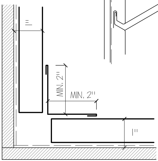
3 INSIDE CORNER DETAIL NTS
